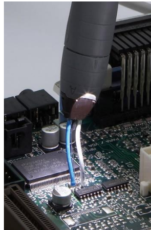
N2750A with solder-in tip
